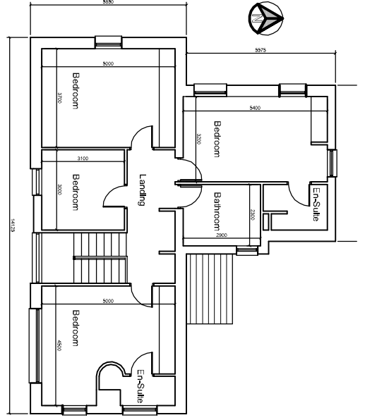
FIRST FLOOR PLAN Area 5.1: 525.9sqm
