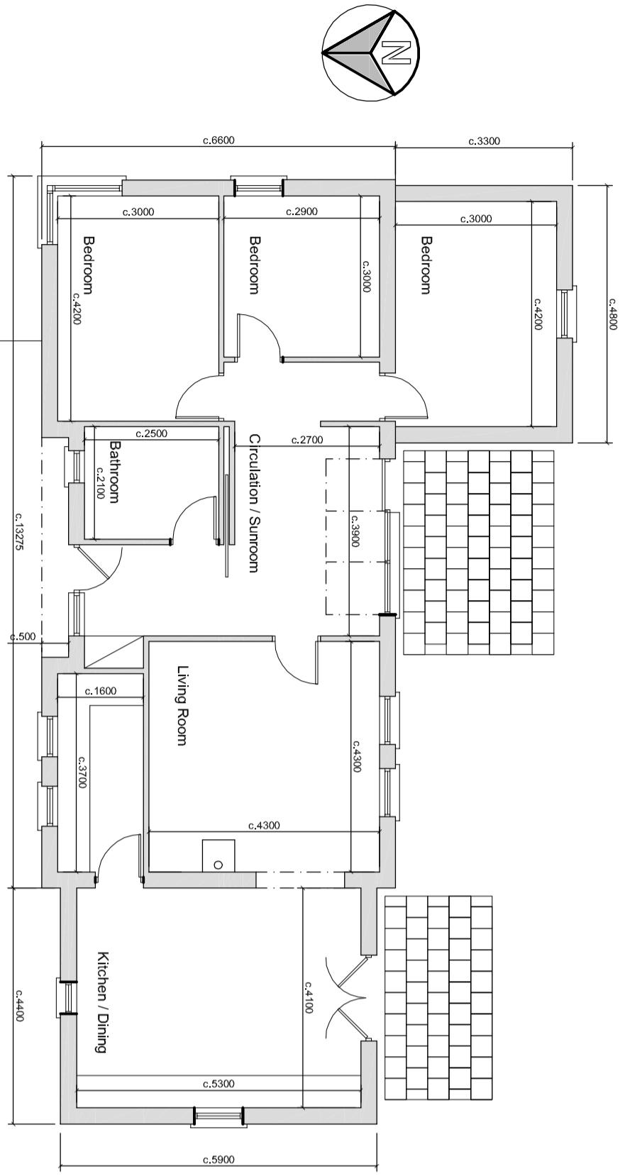
GROUND FLOOR PLAN Floor Area c. 110.5 sq.m (c. 1190 sq ft)
