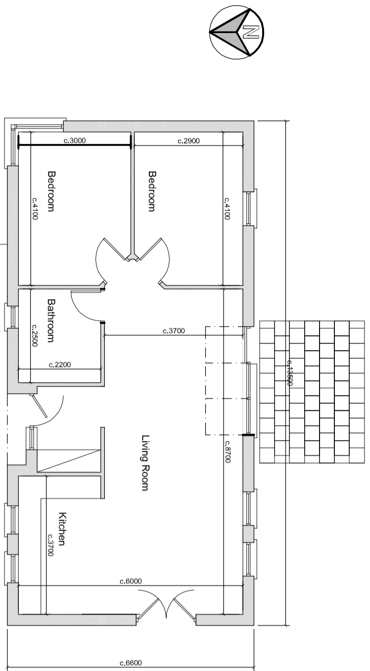
GROUND FLOOR PLAN Floor Area c.76.15 sq.m.(c.819.7 sq ft)
